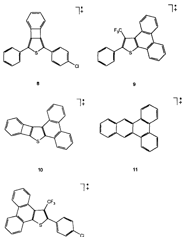
Fig. 1. Polycyclic ions formed in MS analyses.
