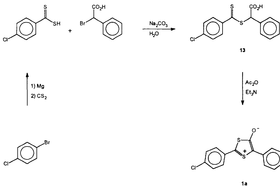
Scheme 3.
