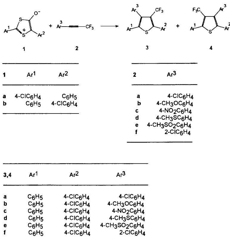
Scheme 1.
